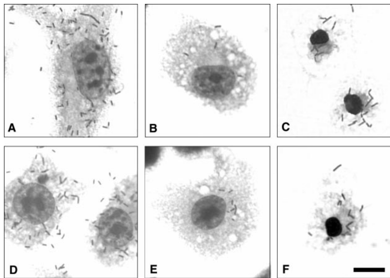
Fig. 2. Light micrographs of J774 macrophages at 6 hours after infection with L. monocytogenes . Each panel depicts a macrophage(s) infected with bacteria producing either (A) wild-type LLO, (B) and (C) LLO \Delta 26, (D) PFO+PEST, or (E and F) PFO-No PEST at an effective MOI of 1:10. In (C) and (F), macrophages were infected in the absence of gentamicin; in all other panels, gentamicin (50 \mu g/ml) was added 30 min after bacterial internalization. Scale bar, 10 \mu m.
