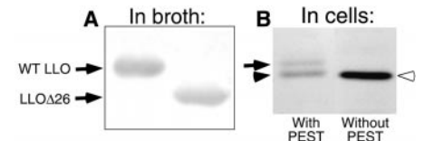
Fig. 3. LLO lacking the PEST-like sequence accumulates to high levels inside, but not outside, of host cells. (A) Western blot showing the relative levels of wild-type and LLO \Delta 26 protein found in the supernatant of bacterial cultures after 5 hours of growth in Luria-Bertani broth. Secreted proteins were isolated as described (8) and subjected to Western blot analysis with polyclonal antibodies raised against LLO. Each lane represents supernatant from equivalent numbers of bacteria. (B) Autoradiograph showing the relative levels of LLO G486D and LLO \Delta 26 G486D recovered from infected macrophages. Bacterial proteins were metabolically labeled with [ 35 S]methionine during growth in J774 cells (7) at 5 hours after infection. LLO was immunoprecipitated as described (7) and subjected to SDS-polyacrylamide gel electrophoresis. Each lane represents a single J774 monolayer ( \sim 4 \times 10^6 cells) that contained 7 \times 10^7 DP-L4044 (LLO G486D ) or 7.7 \times 10^7 DP-L4045 (LLO \Delta 26 G486D ) bacteria. The arrow indicates full-length LLO G486D , the solid arrowhead indicates truncated LLO G486D , and the open arrowhead indicates full-length LLO \Delta 26 G486D .
